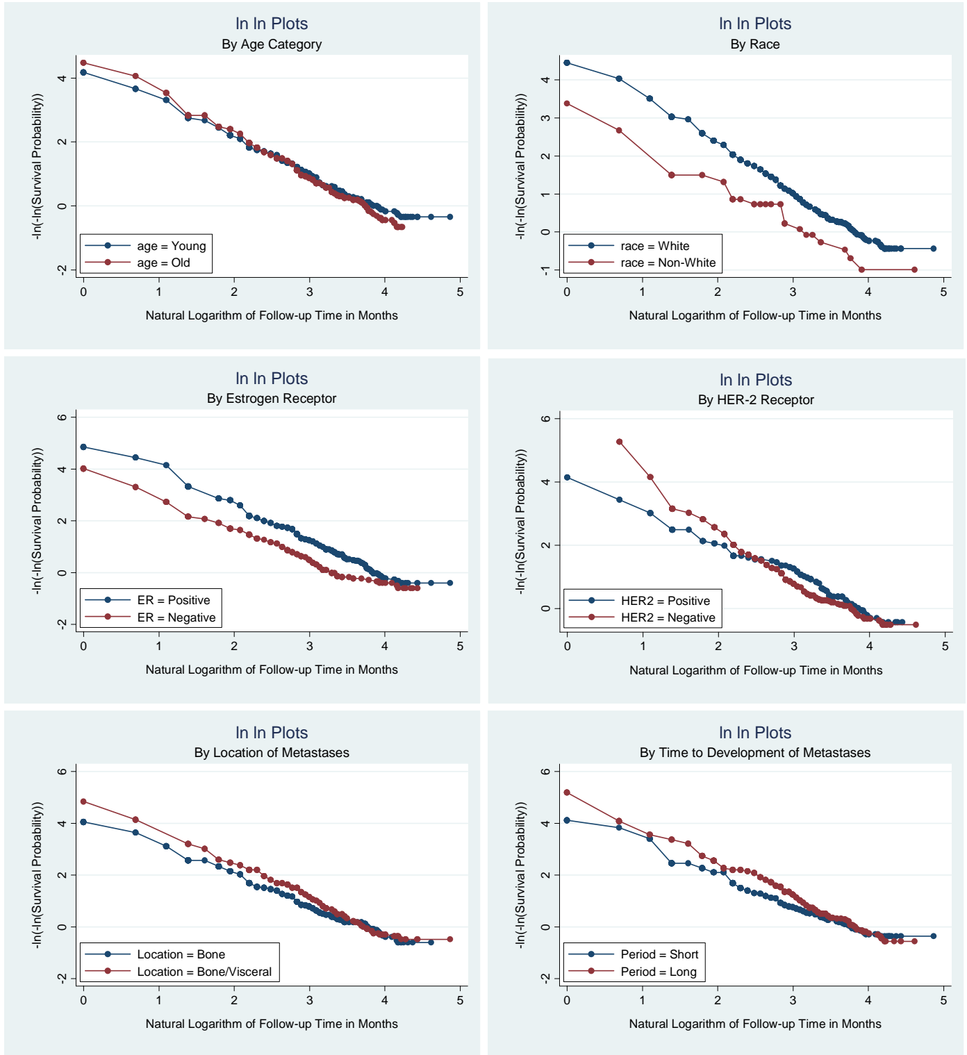
Figure 10. Graphical proportionality assumption test for fixed covariates
