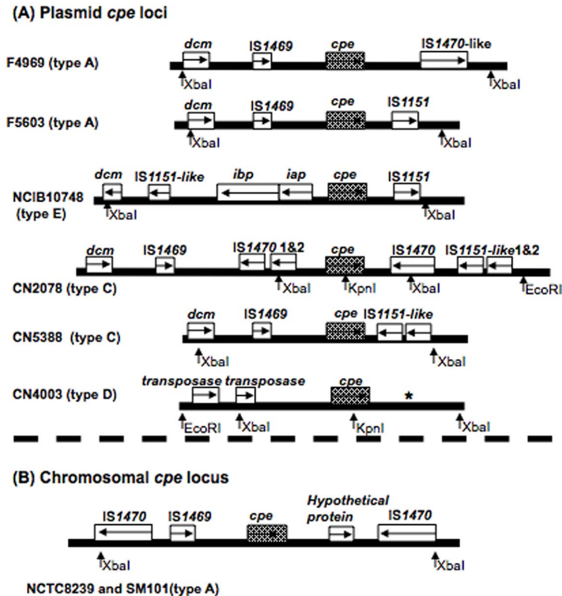
Figure 4. Organization of cpe loci in type A, C, D and E. A) Organization of plasmid cpe loci. B) Organization of the type A chromosome cpe locus. Each box represents an ORF. * indicates a region with sequence similarity to sequences present downstream of cpe in F4969, except for the absence of an IS1470-like gene. Sequences of cpe loci in F4969, F5603, NCIB10748, NCTC8239 and SM101 have been reported previously [11,21,38]. Sequences of CN2078, CN5388 and CN4003 are based upon results of this study. The arrows show predicted enzyme (EcoRI, XbaI and KpnI) cleavage sites used in this study. doi:10.1371/journal.pone.0010932.g004
