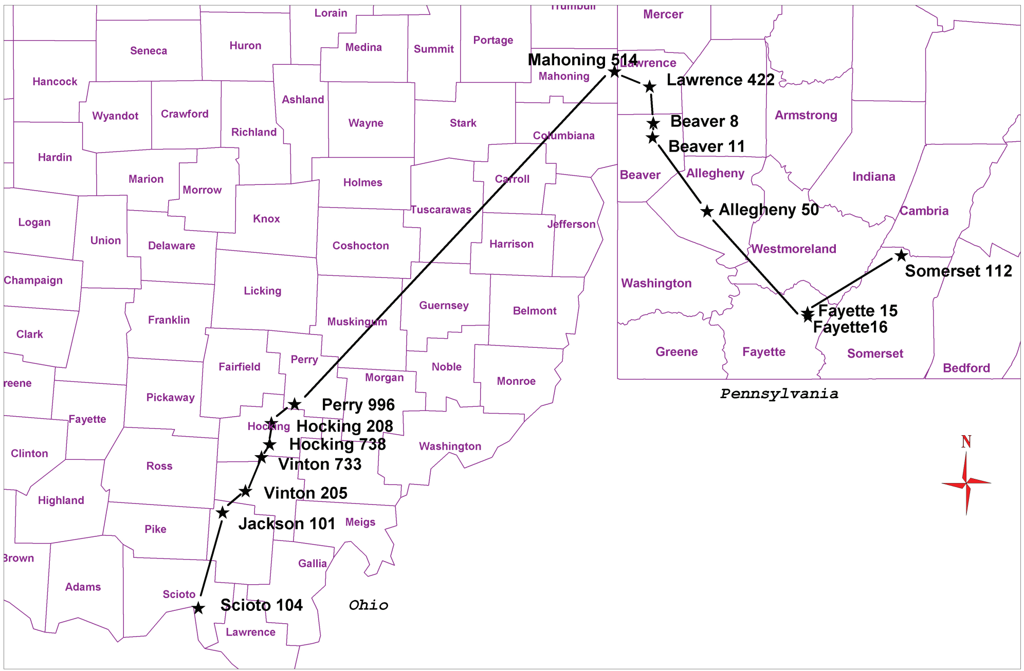
Location of Stratigraphic Sections
