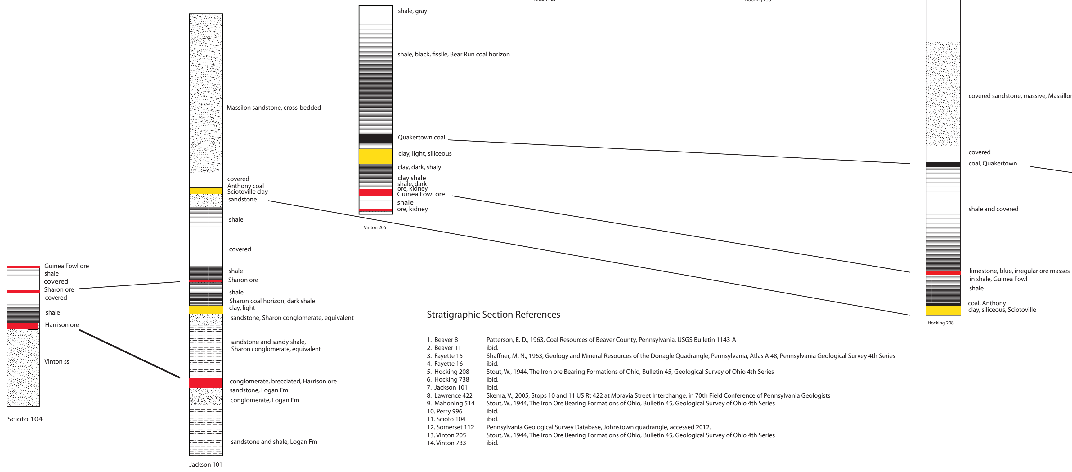
DISTRIBUTION OF COGENETIC IRON AND CLAY DEPOSITS IN THE CENTRAL APPALACHIAN REGION M. S. THESIS MARY K. MCGUIRE MAY 20, 2012
