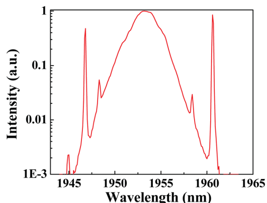
FIG. 3. Typical spectrum of the mode-locked laser on logarithm scale.
