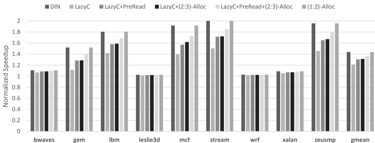
Figure 11: System performance under different schemes (normalized to baseline , bigger is better).
