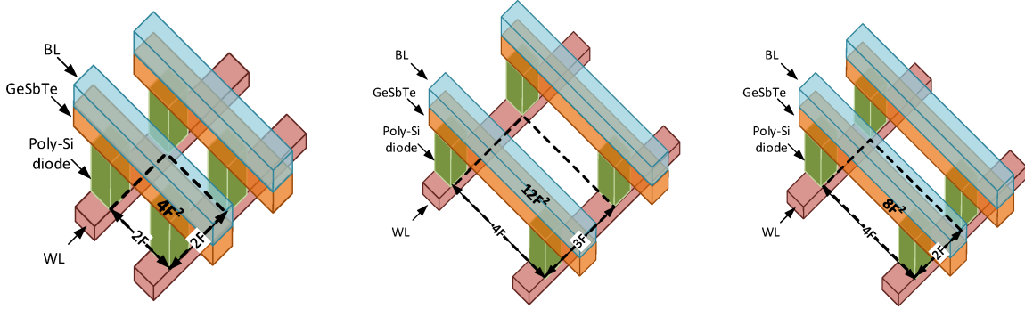
(a) Ideal super dense chip ( 4F^2/\text{cell} ) (b) Prototype chip [8] ( 12F^2/\text{cell} ) (c) DIN[10]-enhanced chip ( 8F^2/\text{cell} )
