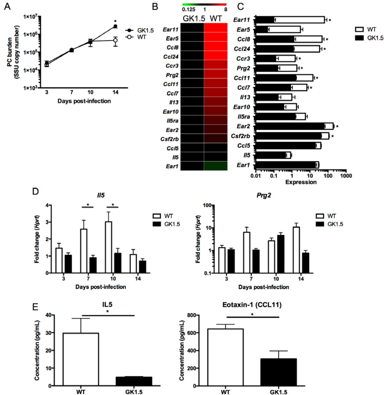
Figure 2-1. RNA sequencing of whole lung shows a prominent CD4-dependent eosinophil signature at day 14 of Pneumocystis infection.
