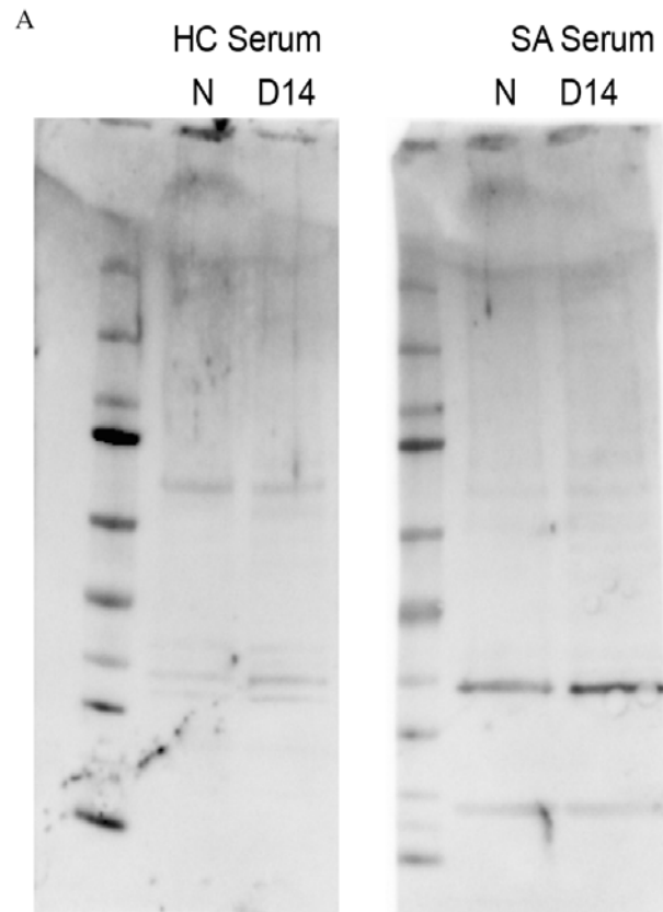
Figure 3-13. Serum from a healthy control and severe asthma patient demonstrate limited reactivity to mouse lung protein.
