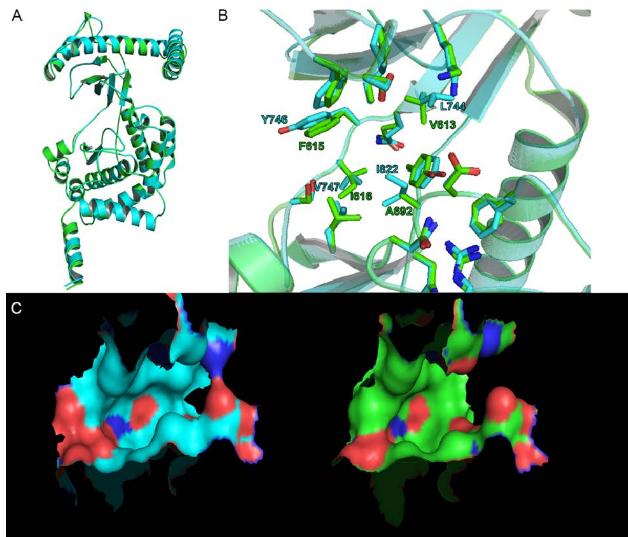
Figure 5-8. Modeling of the Pneumocystis VPS34 binding pocket.
