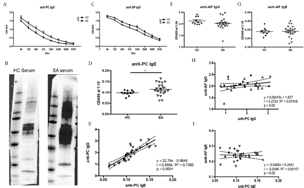
Figure 3-12. Patients with severe asthma have elevated anti- Pneumocystis IgG and IgE levels.
