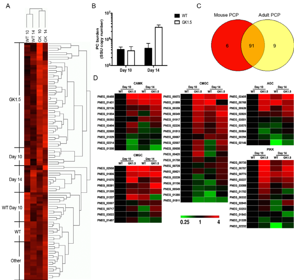
Figure 5-6. Figure 4. The Pneumocystis kinome is expressed during models of infection and during clinical infection.
