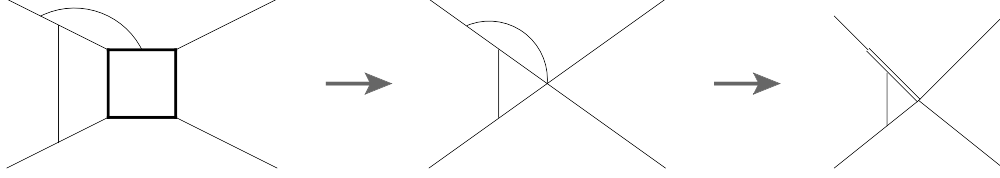
Figure 4: Construction of a physical spacetime diagram. The bold lines are off-shell. They are shrunk to a point to form the reduced diagram. The remaining on-shell lines are drawn as straight lines to form the physical spacetime diagram.
