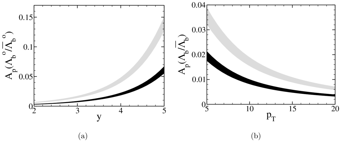
Figure 15: Asymmetry in \Lambda_b^0/\bar{\Lambda}_b^0 production as a function of (a) rapidity y and (b) transverse momentum p_T in the kinematic region 2 < y < 5 and 5 \text{ GeV} < p_T < 20 \text{ GeV} in 7 TeV (grey band) and 14 TeV (black band) pp collisions.
