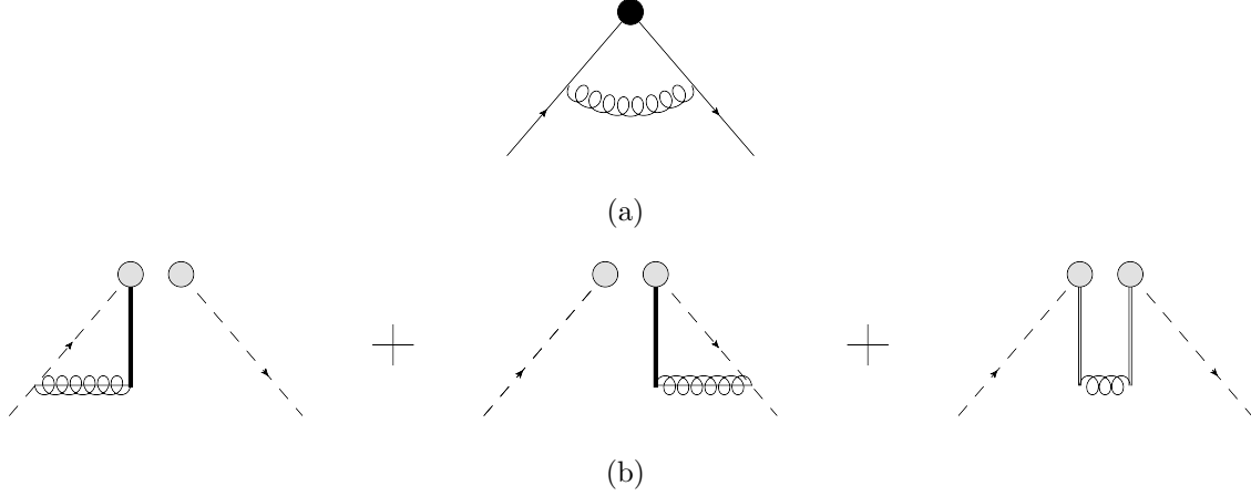
Figure 22: Matching of the QCD current J_V^\mu (a) to the SCET current (b) at NLO. The Collinear Wilson lines and ultrasoft Wilson lines are denoted by bold lines and double lines respectively.
