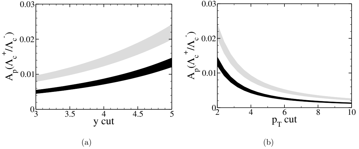
Figure 16: Integrated asymmetry in \Lambda_c^+/\Lambda_c^- production as a function of (a) upper y cut and (b) lower p_T cut in the kinematic region 2 < y < 5 and 2 \text{ GeV} < p_T < 20 \text{ GeV} in 7 TeV (grey band) and 14 TeV (black band) pp collisions.
