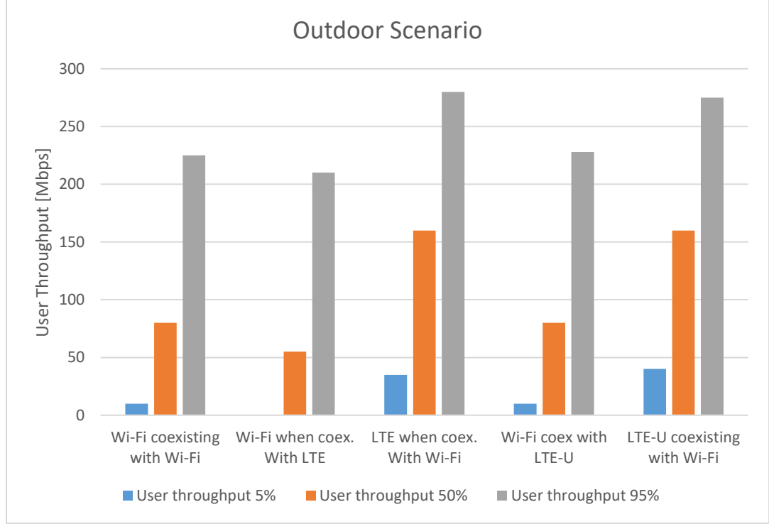
Figure 5. LTE-U and Wi-Fi performance for the Outdoor Scenario for different user throughput loads.
