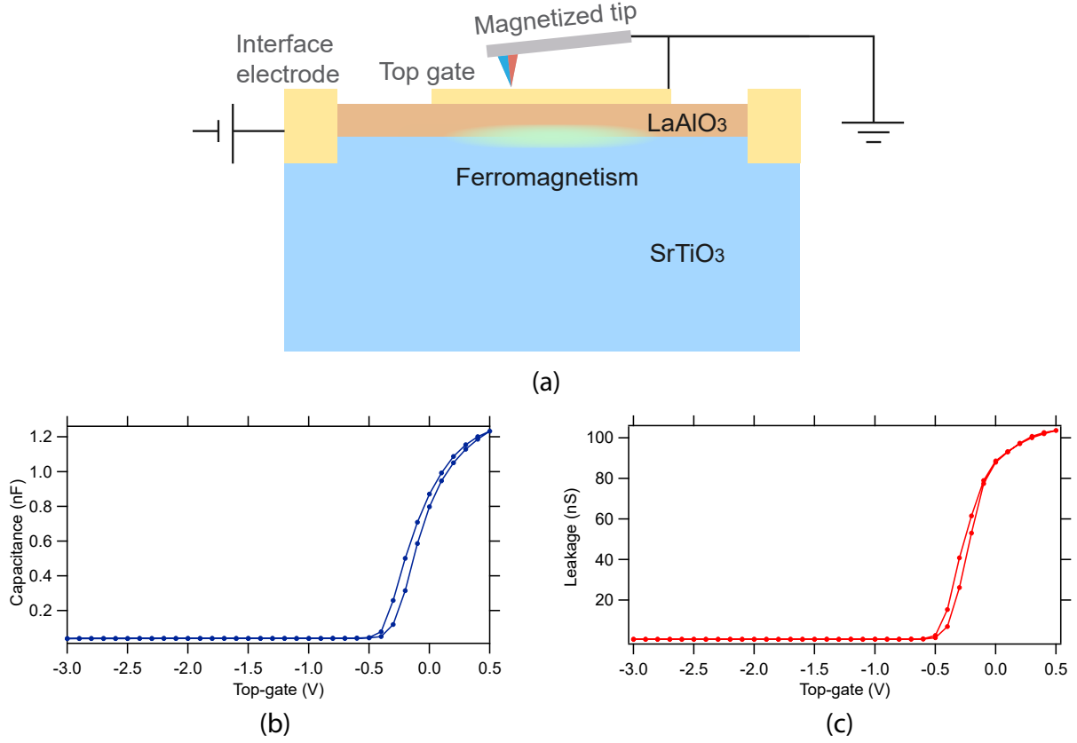
Figure IV.2: (a) MFM experiment setup. The sample within the ferromagnetism thickness window of LAO (8 \mu\text{m} to 25 \mu\text{m} ) is patterned with a top gate electrode and interface electrode. The top gate is connected with the conductive MFM tip and grounded. The interface and top gate form a capacitor. A positive voltage of +1 V to +3 V is applied to the interface, and the interface electrons are depleted. The MFM tip coated with 50 nm of Co/Fe alloy is magnetized in the in-plane direction. When gate voltages deplete the itinerant electrons, the ferromagnetism is visible from MFM measurements. (b) and (c) are the capacitance and leakage current between the interface and top gate, as functions of relative voltage between the interface electrode and top gate. The top-gate voltage in the figures is equal to the potential on the top gate (grounded) minus the potential on the interface. When the top-gate voltage is lower than -0.5 V, both the capacitance and leakage are close to zero, meaning the interface carriers are depleted.
