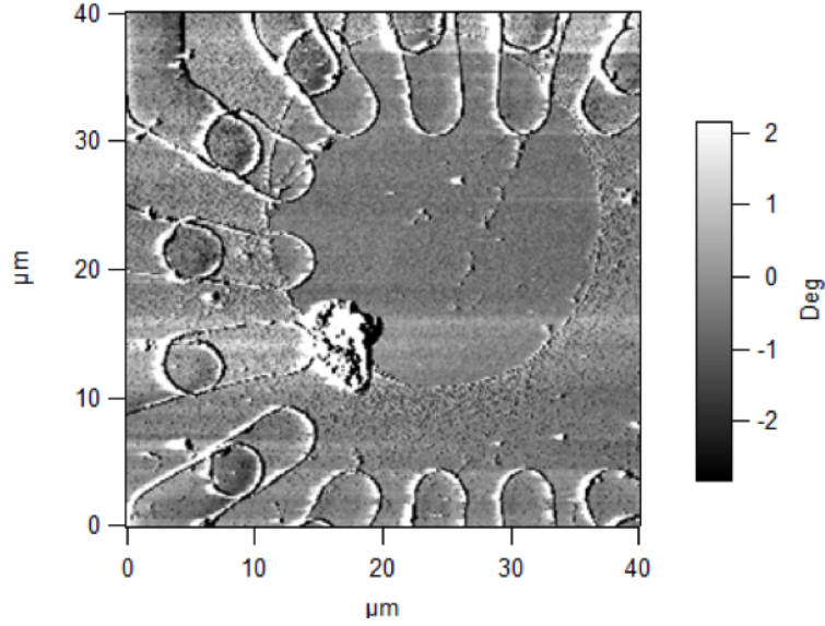
Figure II.25: AFM phase image of graphene on LAO/STO, transferred with PMMA. The circular region is graphene. Particles can be seen outside graphene, on LAO/STO surface. Other features are the metal electrodes for graphene and interface contact.
