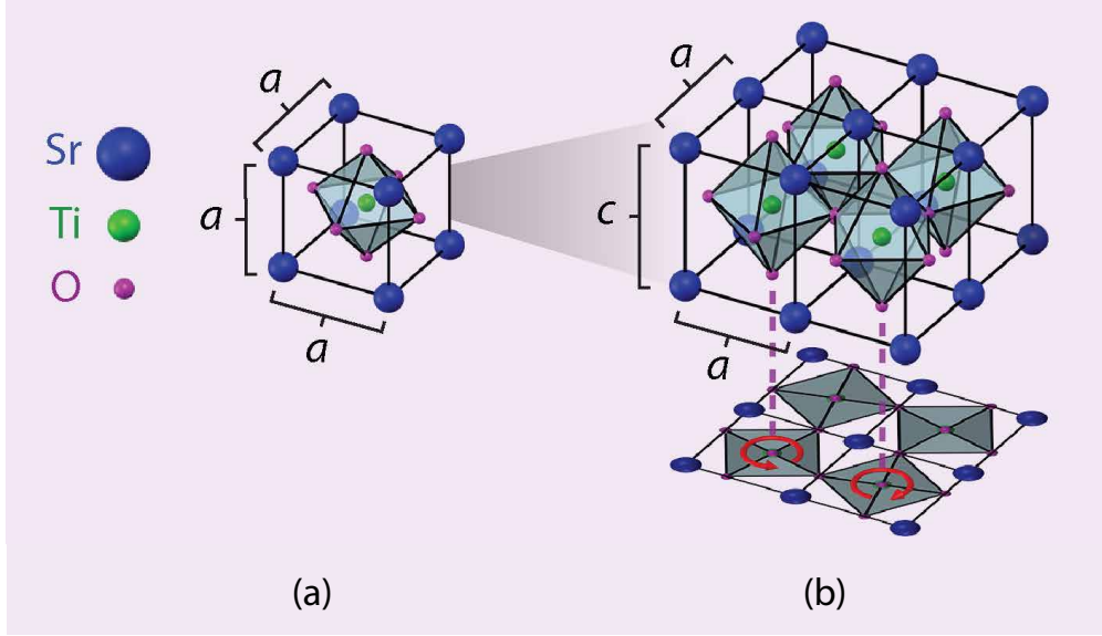
Figure I.1: Ferroelastic transition of STO. (a) At T = 300 K STO has cubic perovskite structure. (b) At T = 105 K, the adjacent oxygen octahedrons would rotate in opposite directions and cause ferroelastic transition in STO. Domains will be formed for different orientations of unit cells. Adapted from [45].
