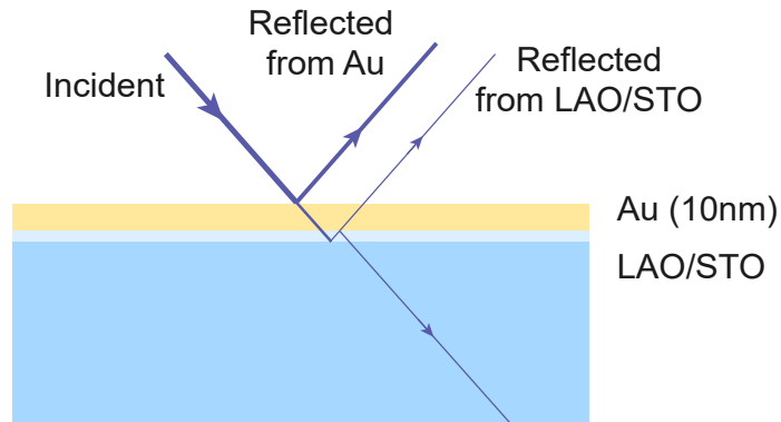
Figure IV.10: Incident and reflected light from LAO/STO need to transmit through the Au top gate.
