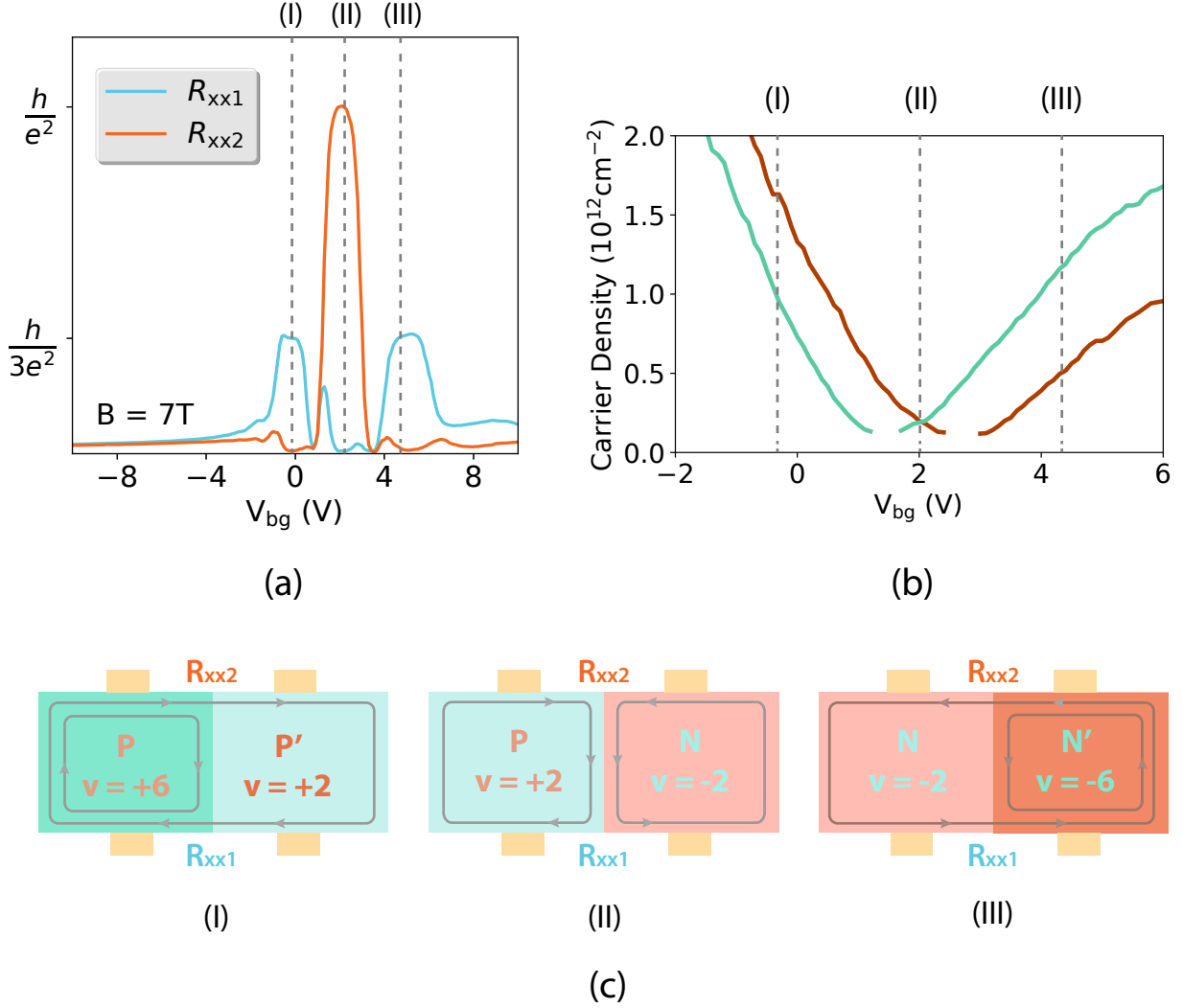
Figure III.15: The edge channel mixing changes as V_{bg} is swept from -10\text{ V} to +10\text{ V} . (a) R_{xx1} and R_{xx2} are quantized at values predicted by equation III.3 and III.6. (b) Zoomed-in plot of Figure III.13. (c) Filling factors and edge current directions of the three cases of edge state mixing. Adapted from [130].
