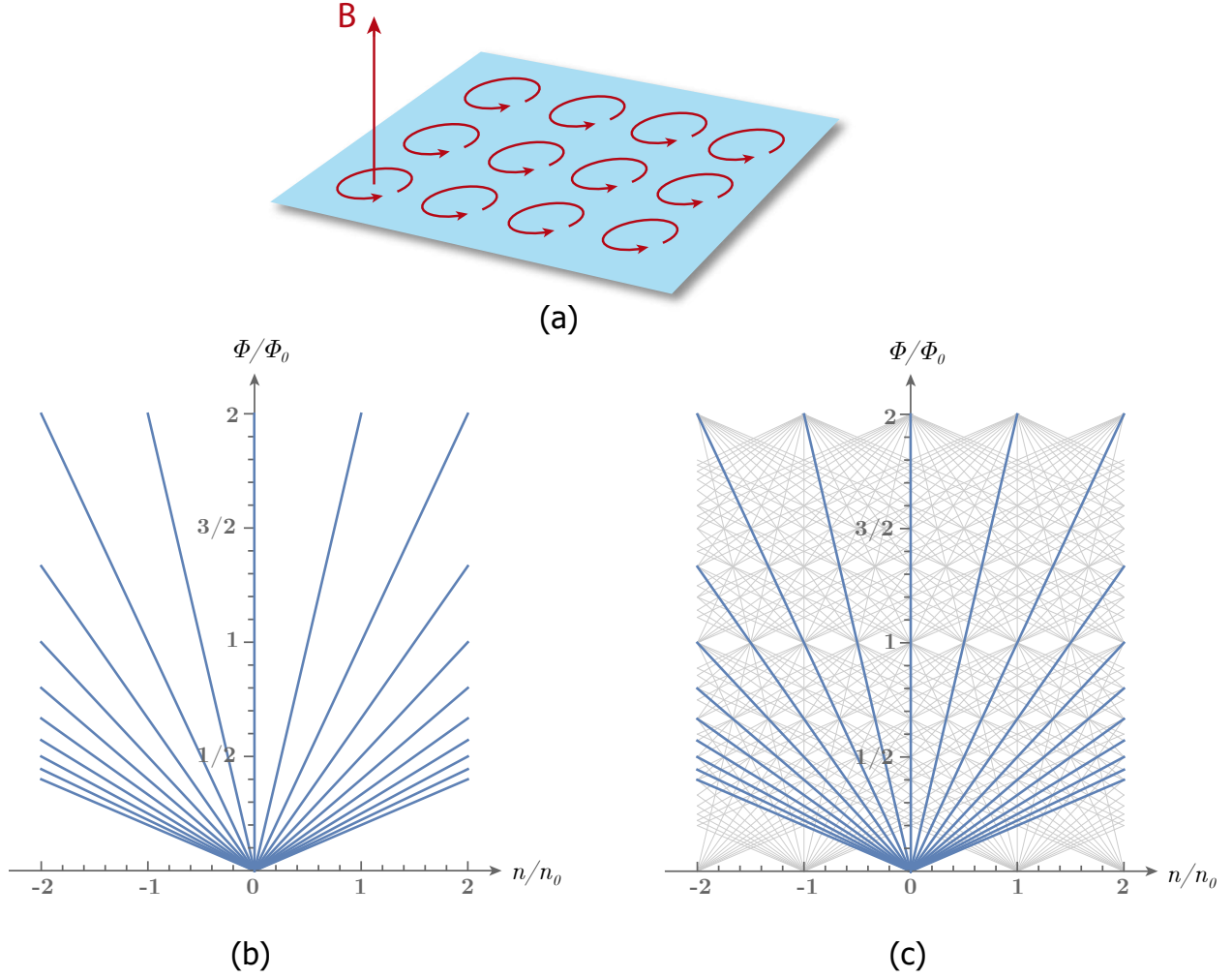
Figure III.18: Landau levels and Hofstadter spectra. (a) Magnetic flux through the electron orbits in magnetic field is quantized. (b) Landau fan diagram of the energy gaps in 2D system. (c) Additional Landau fans emerge under the periodic potential. The energy gaps can be described by equation III.7.
