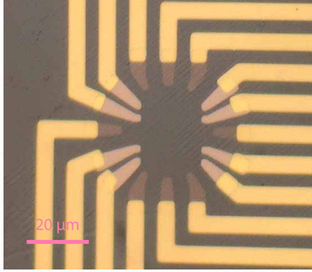
Figure II.31: The graphene area of interest on pre-patterned LAO/STO sample. The patterns are for graphene and LAO/STO interface contact.
