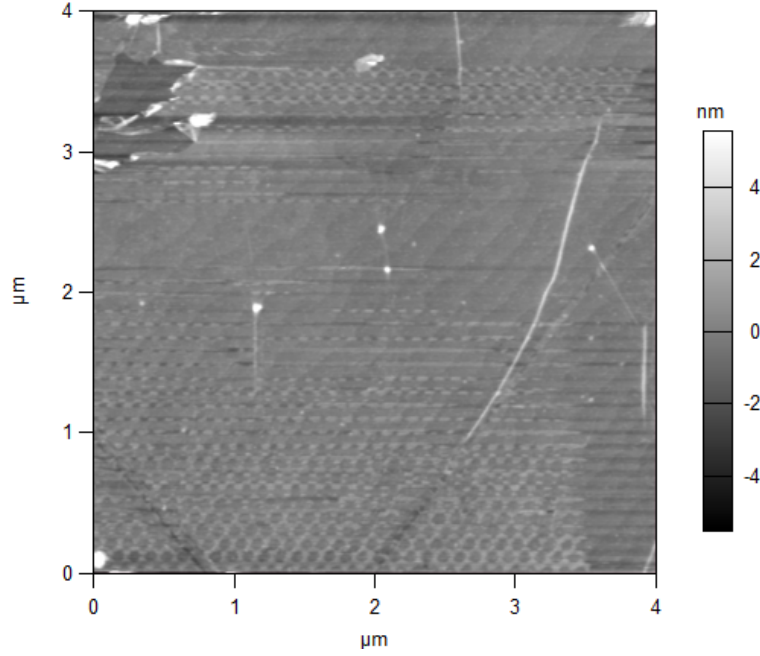
Figure III.21: The topographical change of graphene after superlattice c-AFM writing. The superlattice pattern written on the graphene is visible on the topography image, and cannot be erased by negative tip voltages, suggesting that permanent structural changes have been caused by c-AFM writing.
