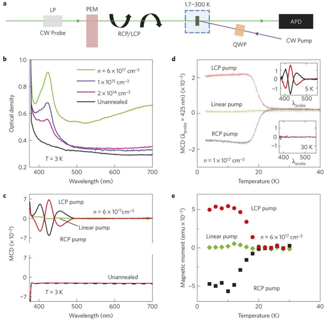
Figure IV.1: MCD experiment on oxygen-deficit STO. (a) The schematics of the optical setup of MCD. (b) An additional peak at \lambda = 425 nm is observed in the absorption spectra of the oxygen-deficit STO samples. (c) MCD spectra of oxygen-deficit and as-received samples after illuminated by circular and linearly polarized pump laser. (d) Temperature dependence of the MCD signal. (e) Temperature dependent magnetic signal measured by SQUID. Adapted from [164].
