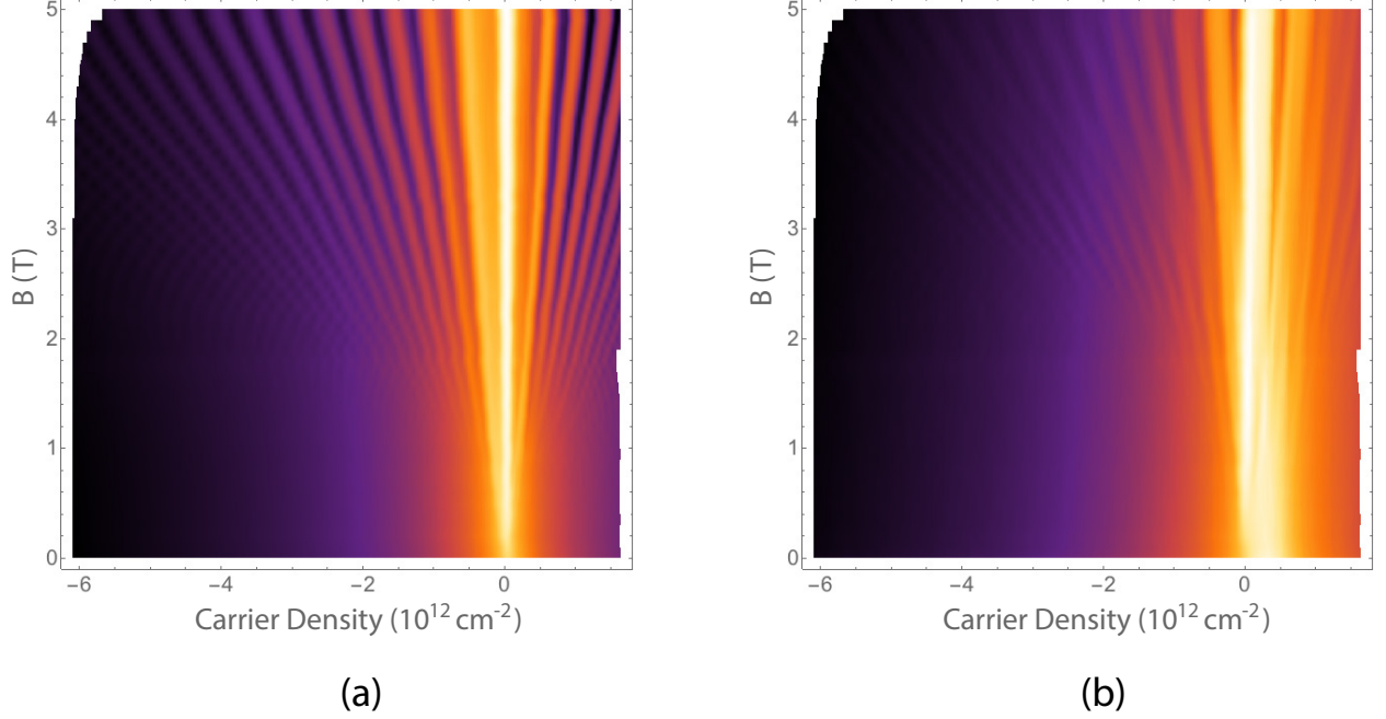
Figure III.20: Longitudinal resistance of the control and written devices ( R_{xx1} and R_{xx2} in Figure III.19(a), in log scale). (a) For the control device, the Landau levels are further apart as the out-of-plane magnetic field increases, and the longitudinal resistance shows a Landau fan diagram. (b) In the graphene with a superlattice written with c-AFM, additional Landau levels are generated from the superlattice and cross the original Landau levels from graphene.
