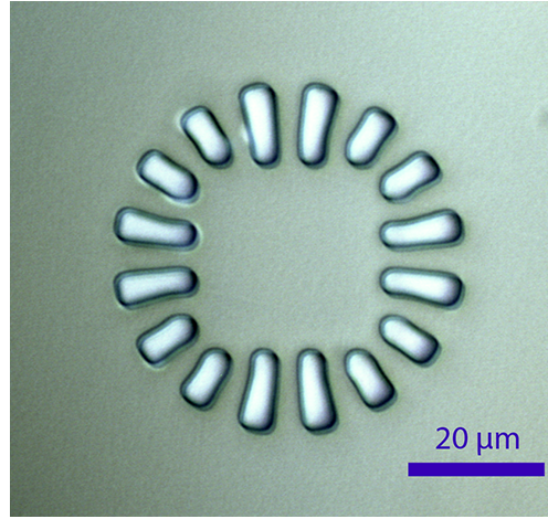
Figure II.12: Exposed and developed sample. The bright regions are free of photoresist while the rest of the sample is still covered.
