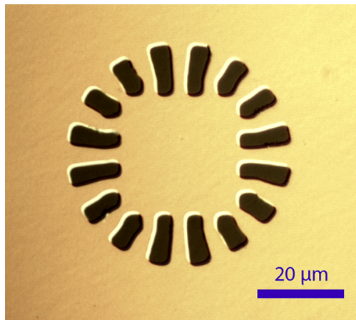
Figure II.9: Mask for photolithography. The dark regions are transparent, while the bright regions are covered with chromium. The sample is exposed where UV is not blocked by chromium. The figure shows the electrodes of a canvas for c-AFM writing.
