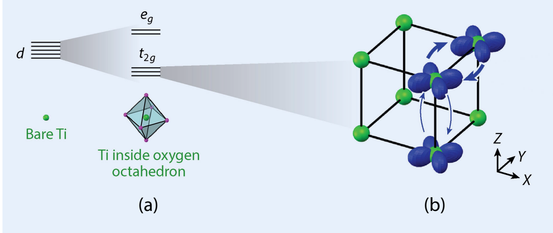
Figure I.2: The band structure of bulk STO. (a) The conductive bands derive from the 3d orbitals of Ti. The degeneracy of the orbitals is broken by the octahedral cage of oxygen atoms, and the energy levels are grouped into e_g and t_{2g} . (b) The hopping of d_{xy} , d_{xz} and d_{yz} are much easier along in the plane directions, mediated by the 2p orbitals of oxygen atoms. Adapted from [45].
