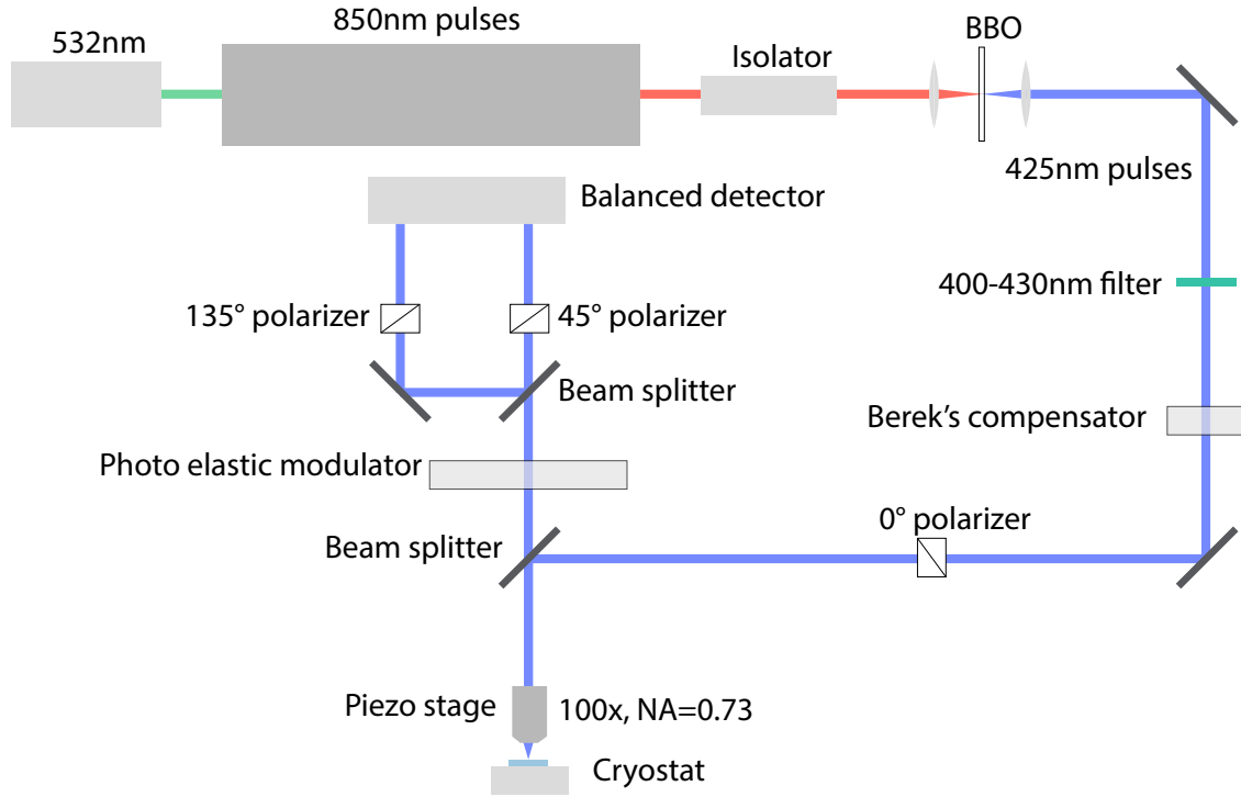
Figure IV.6: The Kerr rotation measurement optics. \lambda = 850 nm pulsed laser is generated from a Tsunami oscillator, at 78 MHz repetition rate and 150 fs duration. The laser frequency is doubled with BBO. \lambda = 425 nm laser passes through a band-pass filter and is then horizontally polarized. The laser is focused onto the sample with a 100 \times objective. The reflected laser is modulated by a PEM and then split into two branches that pass through two polarizers at 45° and 135°. The intensity signal is measured with a balanced detector.
