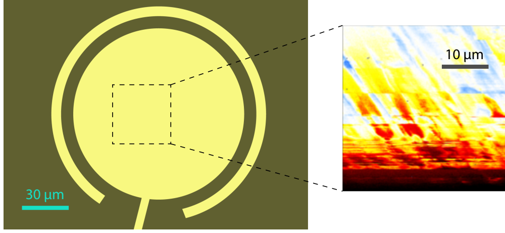
Figure IV.3: Optical image of the MFM device and MFM signal for interface magnetism. The circular shape region is the top gate, and the arc-shaped electrode is the interface electrode. MFM image is scanned on a 30\ \mu\text{m} \times 30\ \mu\text{m} region on the top gate while the electrons are depleted. Diagonal strips are visible in the MFM image.
