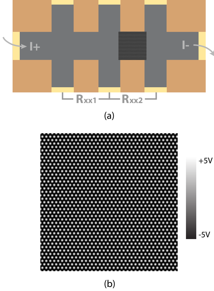
Figure III.19: Lithography of hexagonal superlattice on graphene. (a) The written and control devices. (b) The hexagonal pattern of superlattice, with V_{\min} = -5 V and V_{\max} = +5 V. The pattern is generated using equation III.8.
