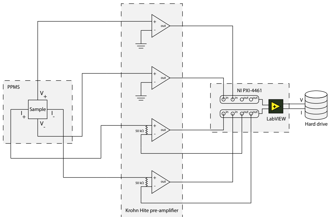
Figure B1: Circuit diagram for electronic signal measurement.
