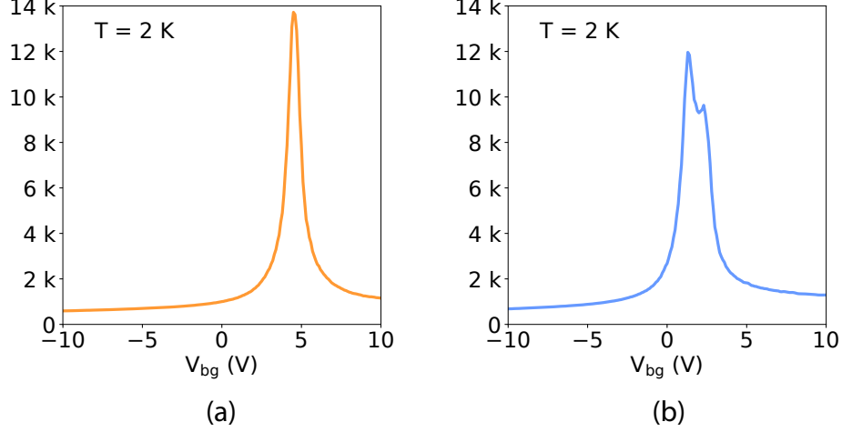
Figure III.14: Longitudinal resistance as a function as V_{bg} . (a) is measured before c-AFM writing as a control measurement. Dirac peak is clearly visible. (b) is measured after c-AFM writing. Splitting of Dirac peak can be observed. The peak on the left hand side is correspond to the written area (shown in the inset of Figure III.13). Adapted from [130].
