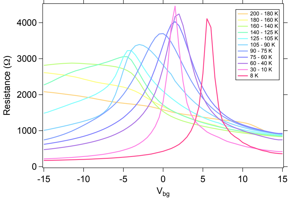
Figure III.4: Resistance as a function of V_{bg} sweep at different temperatures. The width of the CNP clearly shows the change of dielectric constant of STO as a function of temperature.
