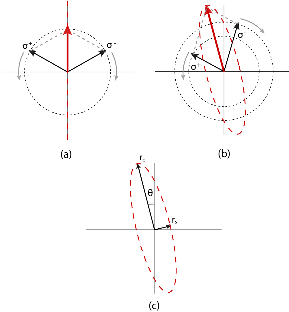
Figure IV.4: Circular decomposition of linearly polarized light and magneto-optical Kerr response. (a) A linearly polarized light can be decomposed into LCP and RCP with equal amplitudes and phases. (b) When the linearly polarized light is reflected from the magnetized surface, the LCP and RCP will end up with different amplitude and phase, and the reflected light is elliptically polarized. (c) the elliptically polarized light is described by rotation angle \theta_k and ellipticity \epsilon_k = r_p/r_s .
