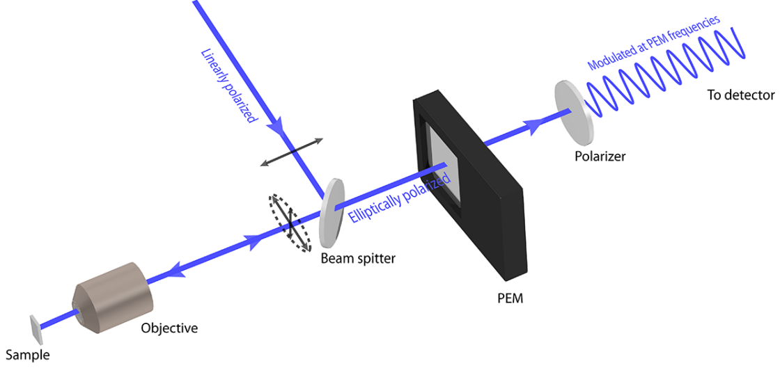
Figure IV.5: The PEM measurement setup. Linearly polarized light is reflected towards the sample and focused by an objective. The reflected light is elliptically polarized and modulated by a PEM. The polarization modulation is converted to intensity modulation and measured by a photodetector.
