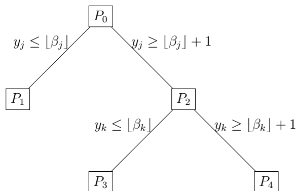
Figure B.4: Branch and Bound algorithm
