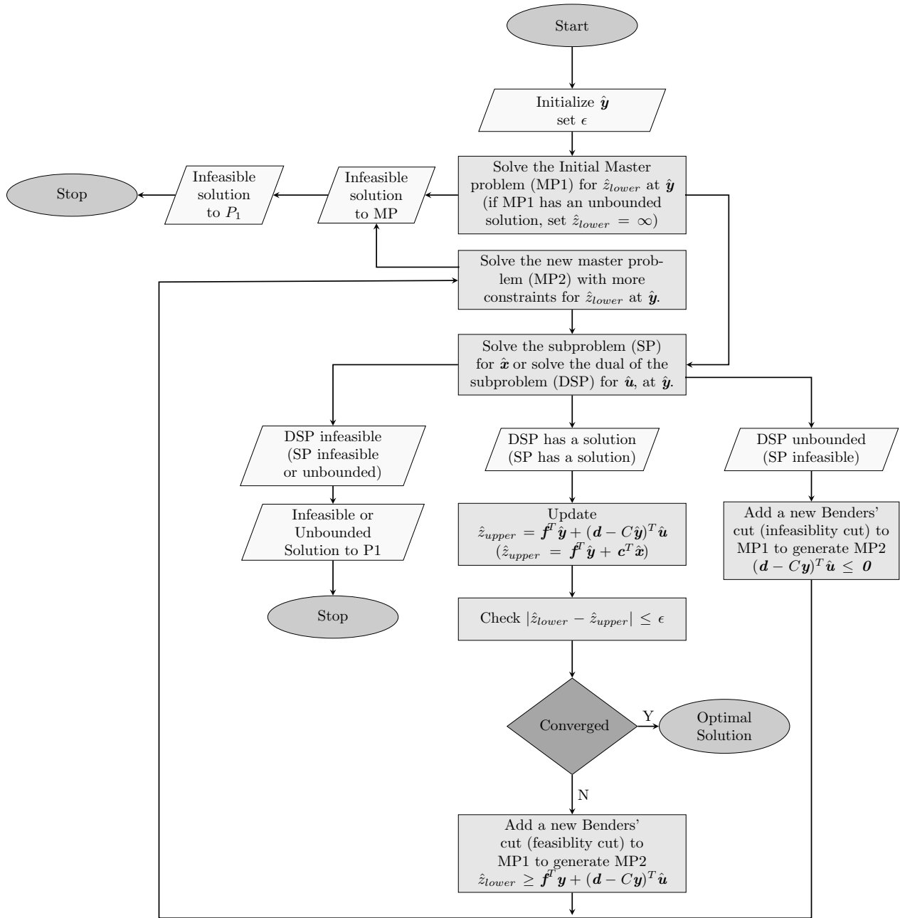
Figure 2: Flowchart of classical Benders' Decomposition algorithm from [30]
