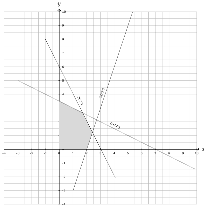
Figure B.1: Gomory cuts
