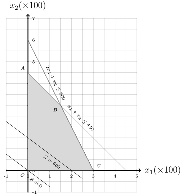
Figure A.1: Feasible region corresponding to Example A.1
