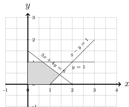
Figure B.3: New feasible region corresponding to Example B.1
