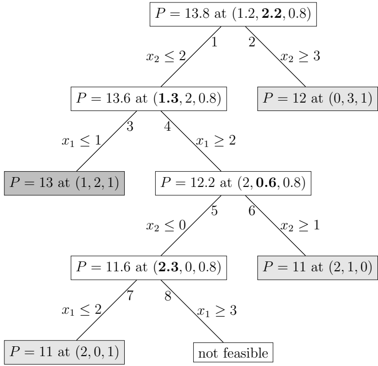
Figure B.5: Process tree corresponding to Example B.2
