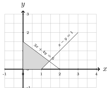
Figure B.2: Initial feasible region corresponding to Example B.1
