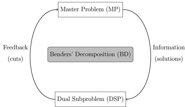
Figure 1: Schematic representation of Benders' Decomposition algorithm from [27]
