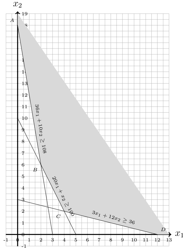
Figure A.2: Feasible region corresponding to Example A.2
