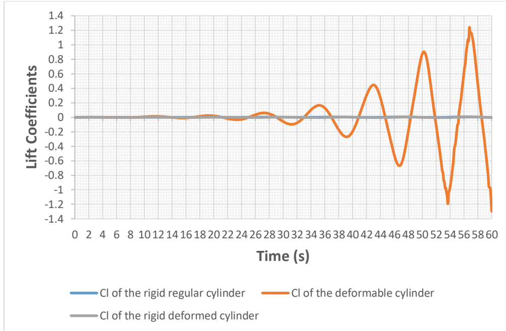
Figure 26. Lift coefficients of Re100
