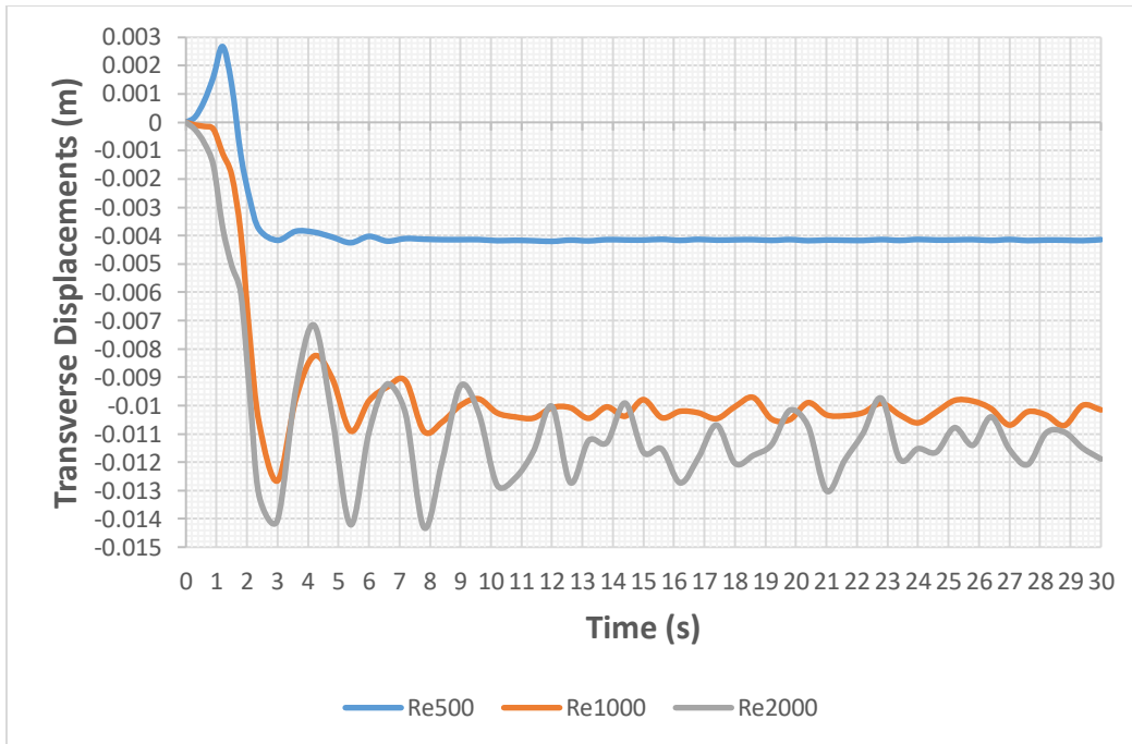
Figure 24. Re500, 1000, and 2000 transverse displacements versus time
