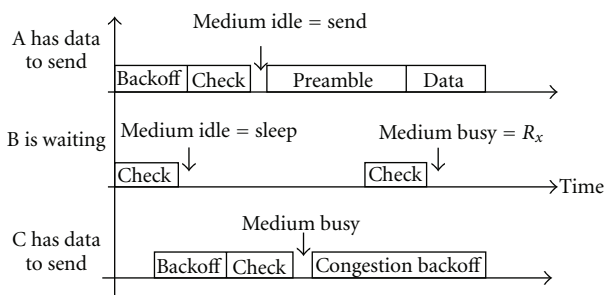
FIGURE 6: B-MAC communication example. All nodes are within range of each other.
