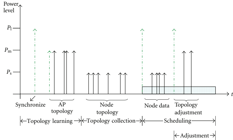
FIGURE 8: PEDAMACS phases: solid arrows are packets sent by nodes; dashed arrows show packets sent by the AP. Different power levels are used in different situations. Only the scheduling phase has defined time slots.
