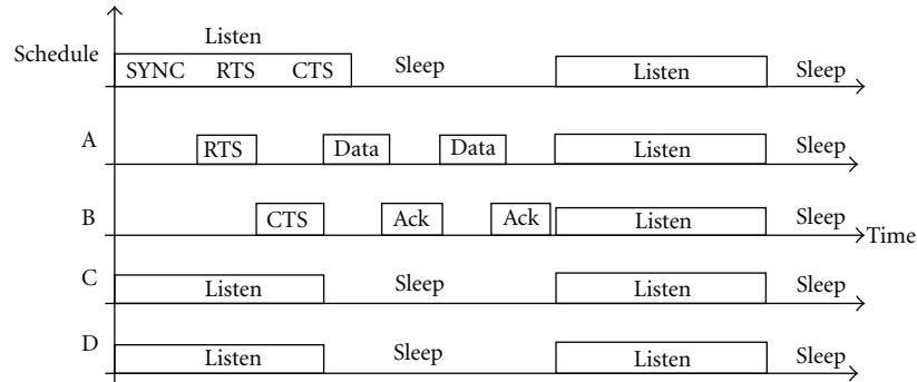
FIGURE 5: S-MAC example. Nodes A, B, and C are within range of each other. D is within range of C and A transmits to B.
