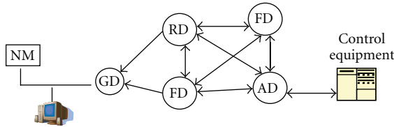
FIGURE 4: Different devices in a WirelessHART network.
