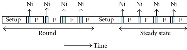
FIGURE 7: LEACH operation rounds. F are frames divided in time slots. Ni are slots assigned to node i .
