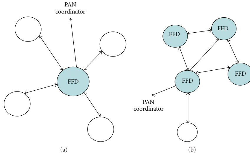
FIGURE 2: (a) Star topology with one full function device and 4 reduced function devices (white circles). (b) Peer-to-Peer topology.
