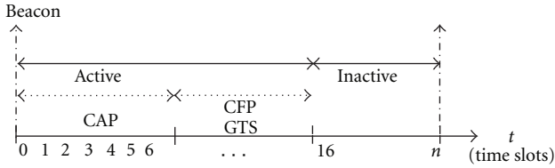
FIGURE 3: Beacon mode structure. Active period has contention (CAP) and noncontention (CFP) modes.
