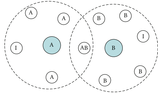
FIGURE 1: Bluetooth scatternet. Shaded circles are master nodes in two different piconets, A and B. White circles show slaves belonging to each piconet. Active slaves are labeled according to the network they belong to; inactive slaves have label I. AB is a slave belonging to both piconets. The figure shows coverage areas of both master nodes.
