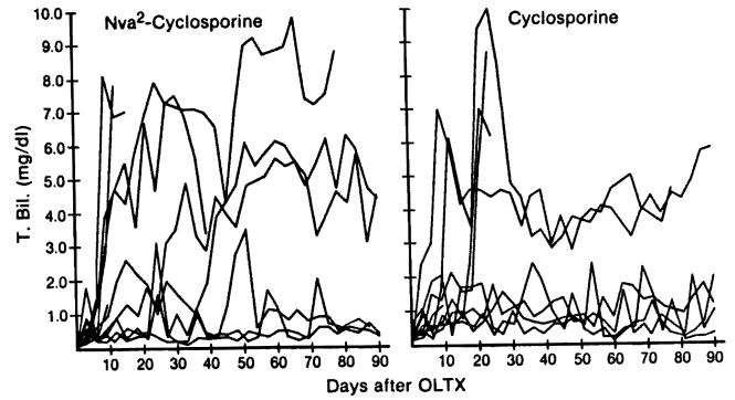
FIGURE 4. Changes in T-bili of group 2 (Nva 2 -CsA) and group 3 (CsA) animals after liver transplantation.
