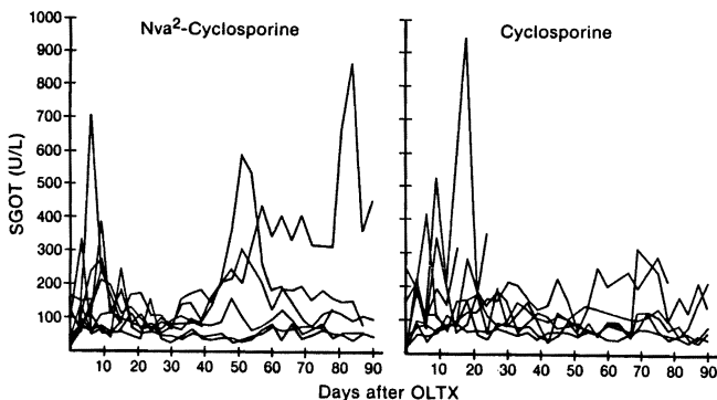
FIGURE 3. Changes in SGOT of group 2 (Nva 2 -CsA) and group 3 (CsA) animals after liver transplantation.
