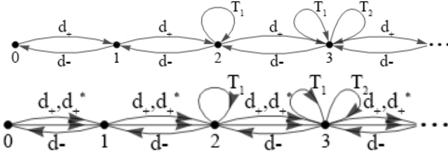
Figure 3: The quivers \dot{\mathbf{Q}} and \ddot{\mathbf{Q}}
