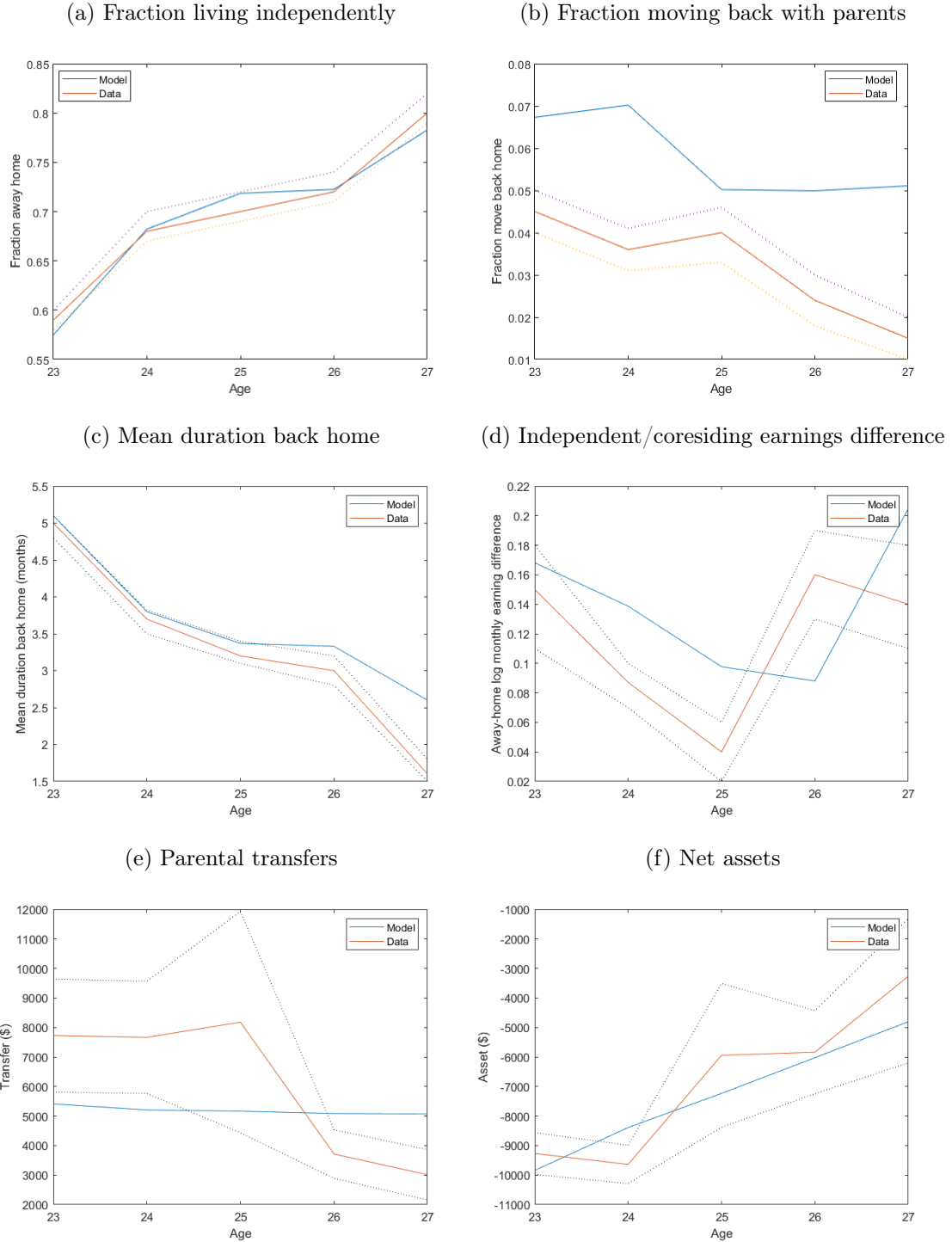
Figure 4: Model Fit
