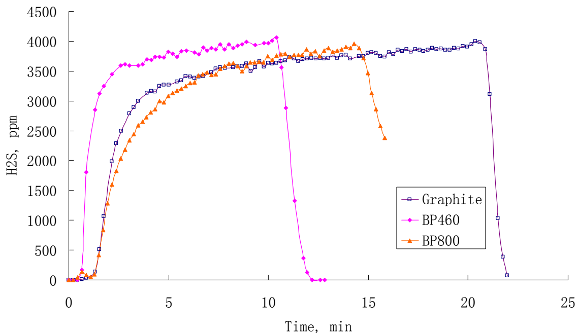
Figure 12. Breakthrough curves of 6 g of carbon black samples (BP460 and BP800) and 12 g of graphite. Sulfurization was performed at room temperature with 4000 ppm \text{H}_2\text{S} under dry condition. The total flow rate of simulated syngas was 0.5 L/min with a space velocity 3800 \text{ h}^{-1} . When the effluent \text{H}_2\text{S} concentration reached 4000 ppm, inlet gas was switched to \text{N}_2 only. By integrating the area above each breakthrough curve, the \text{H}_2\text{S} -uptake capacity could be calculated. The capacity of BP460, BP800 and graphite is 1, 1.29 and 1.41 \text{mg H}_2\text{S/g Sorbent} , respectively.
