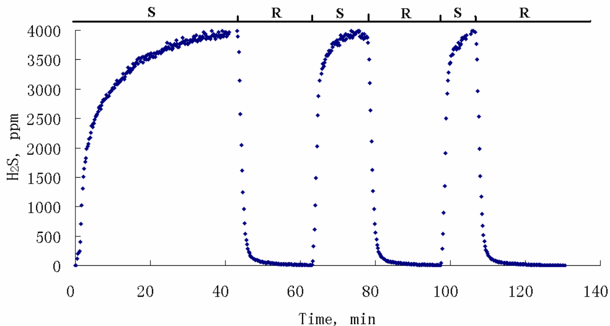
Figure 21. Sulfurization (S) and regeneration (R) of 6 g La 2 O 3 for 3 cycles in order to test the regeneration capability. Sulfurization was performed at room temperature with 4000
