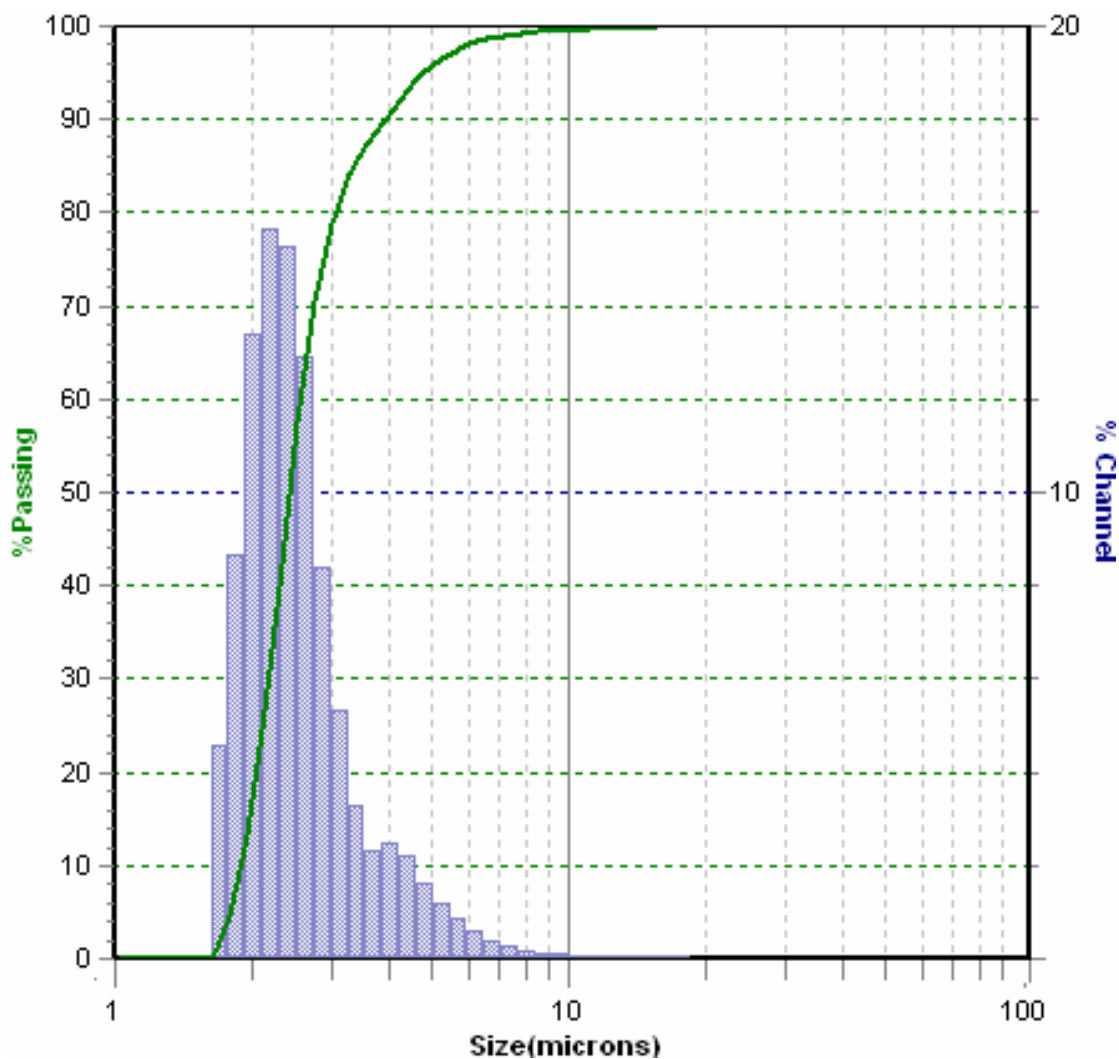
Figure 28. Particle size and distribution of CeO 2 (1.8 – 23 \mu\text{m} ) with an average particle diameter 2.4 \mu\text{m} .
