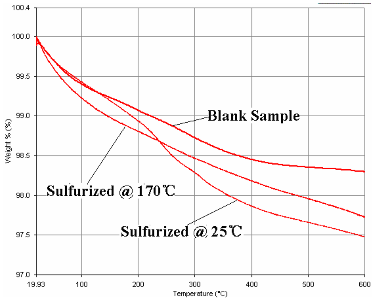
Figure 31. TGA runs of fresh ACF10 without sulfurization and ACF10 after sulfurization. Sulfide samples had more weight loss due to sulfur species retained after sulfurization.
