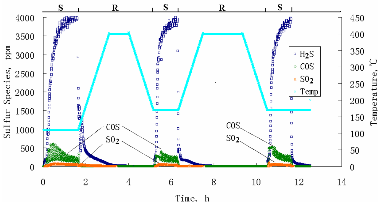
Figure 24. Sulfurization (S) and regeneration (R) of ACF- \text{LaCl}_3 under wet condition. Sulfurization with 4000 ppm \text{H}_2\text{S} , when effluent \text{H}_2\text{S} concentration reached 4000 ppm, simulated syngas was switched to \text{N}_2 , and temperature was increased to 400 °C for regeneration of sorbent. Then temperature was decreased to begin another sulfurization and regeneration cycle. By-product including COS and \text{SO}_2 were also investigated.
