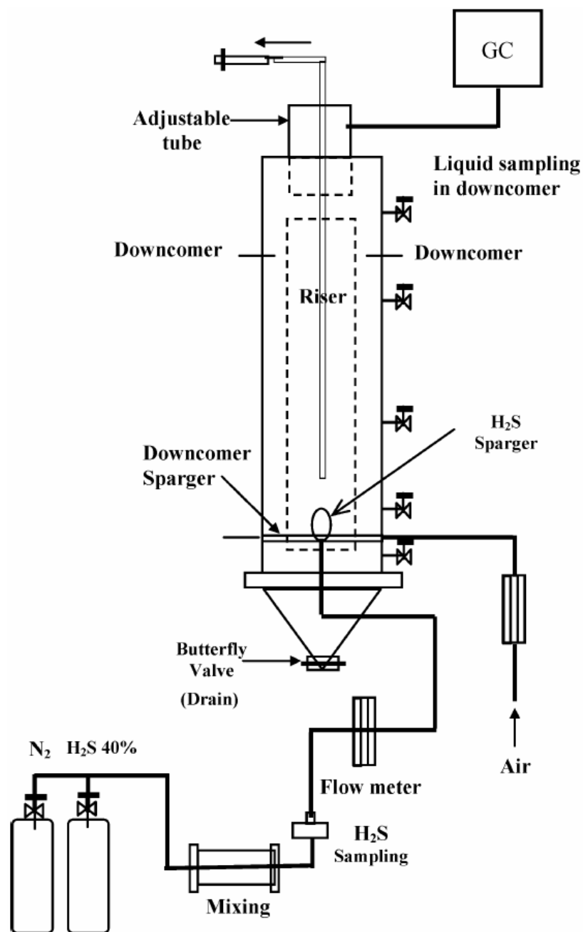
Figure 6. Gas-lift reactor where \text{H}_2\text{S} is injected at the bottom of the riser and air injected in the downcomer for catalyst regeneration. The removal reaction takes place in the riser and regeneration is performed in the downcomer. \text{H}_2\text{S} is injected at the bottom of the riser, where the reaction occurs, and injecting air in the downcomer for catalyst regeneration [39].
