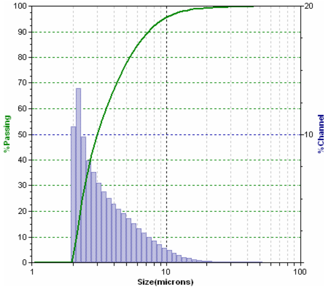
Figure 9. Particle size and distribution of \text{La}_2\text{O}_3 (2.1-68 \mu\text{m} ), with an average particle diameter about 3.04 \mu\text{m} .
