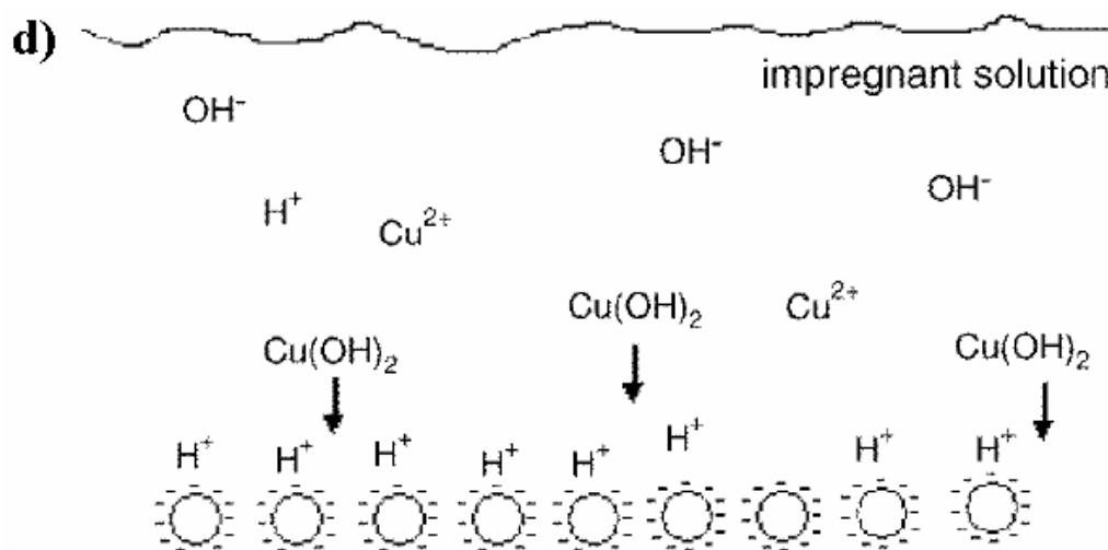
Figure 4. Schematic of movement between impregnated solution and sorbents: a) Copper nitrate dissociates to Cu 2+ and NO 3 - ions in the solution which is used to impregnate activated carbons; b) the negative charge on the surface of unmodified activated carbon attracts H + ions in the solution resulting in pH increase of the solution; c) dissociated Cu 2+ are attracted by activated carbon and combine with OH - to form Cu(OH) 2 ; d) Cu(OH) 2 deposit onto the external surface and inside the pores of activated carbon [9].
