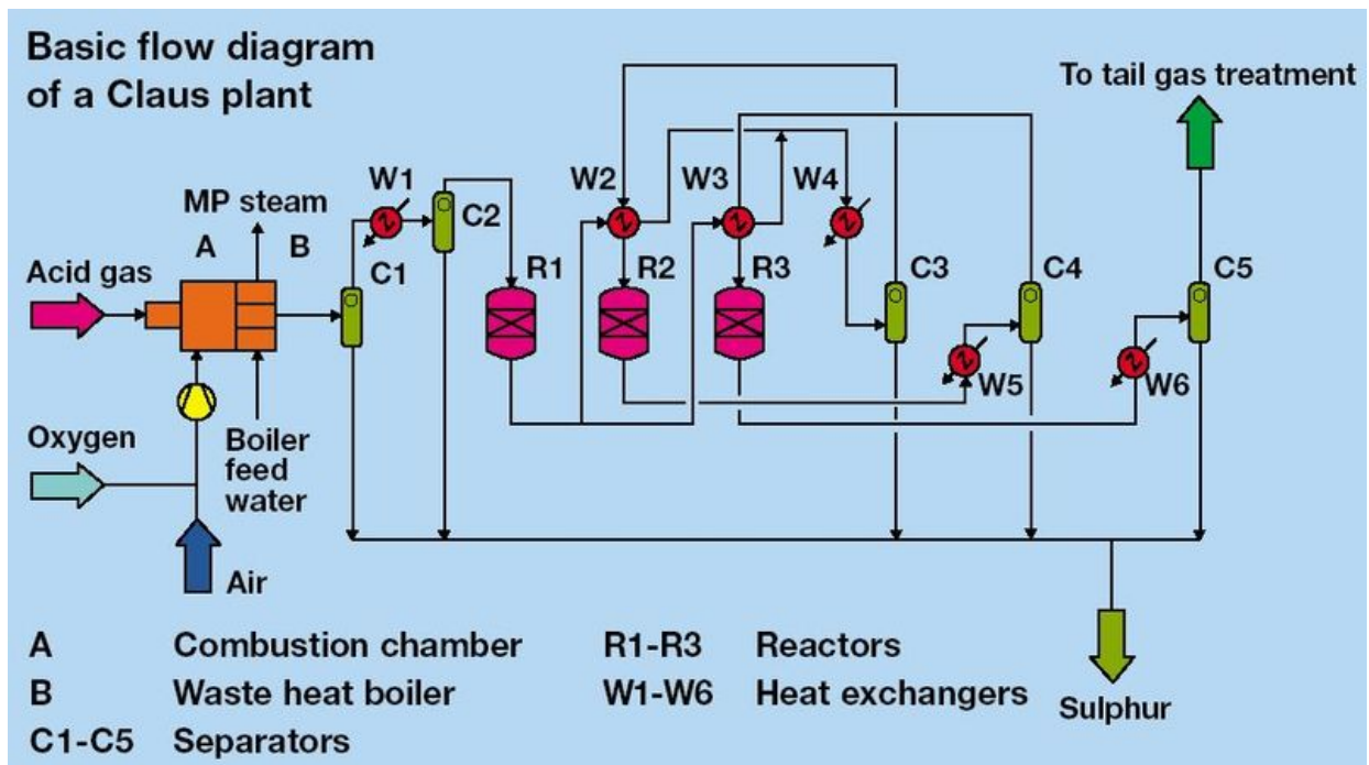
Figure 2. Schematic process flow diagram of a basic Claus process unit. The Claus technology can be divided into two process steps, thermal and catalytic. In the thermal step, \text{H}_2\text{S} -laden gas reacts in a substoichiometric combustion at temperatures above 850^\circ\text{C} such that elemental sulfur precipitates in the downstream process gas cooler. In the catalytic step the process continues with activated \text{Al}_2\text{O}_3 or \text{TiO}_2 , and serves to boost the sulfur yield [17].
