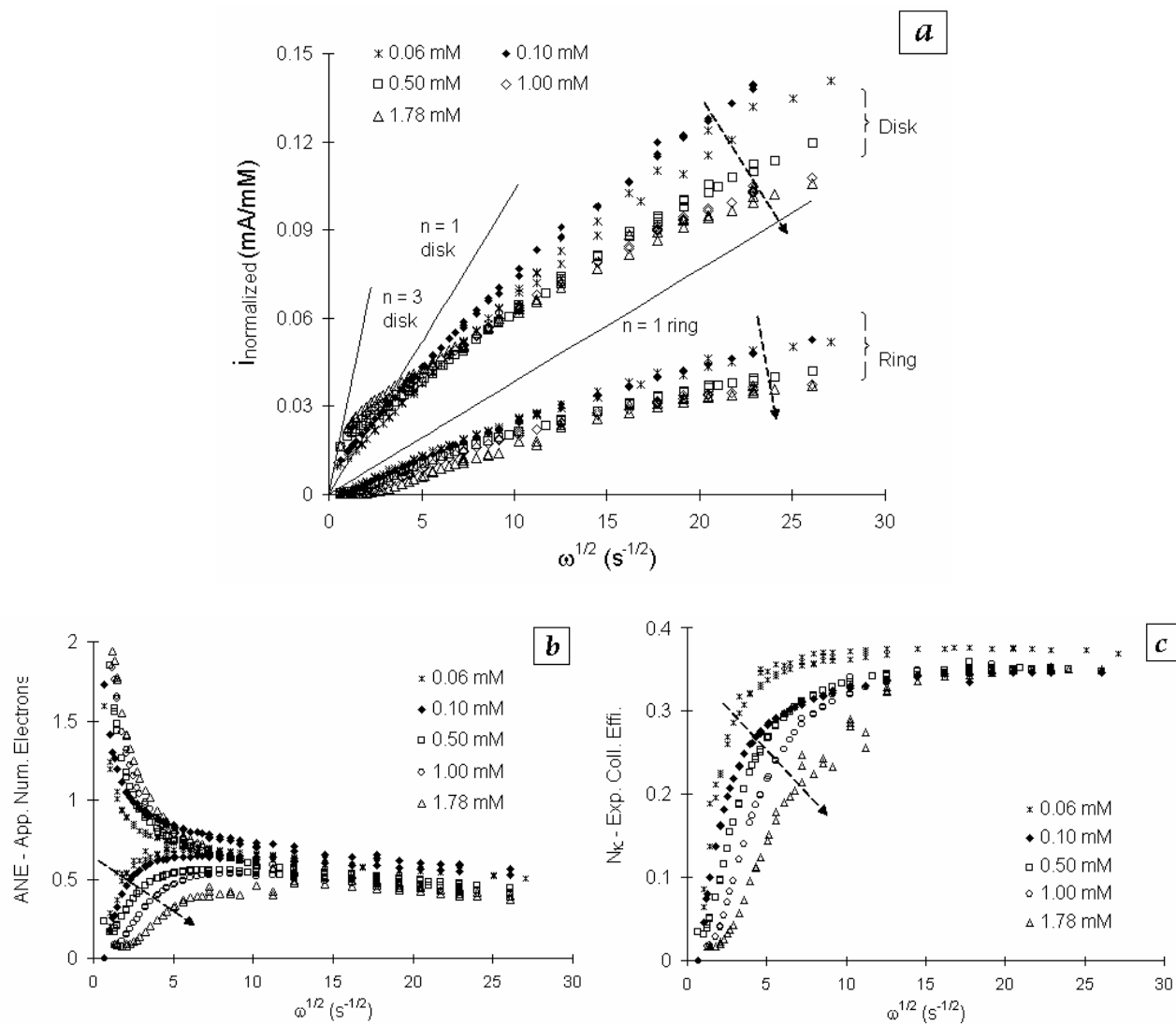
Figure 4-4. Concentration effect on RRDE behavior of 1:1 Cu(II)-TRH.
