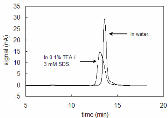
Figure 2-3. Comparison of pre-concentrated TRH signals in SDS-containing solution and water.
