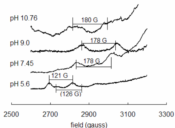
Figure 3-2. The g_{\parallel} region of Cu(II) ESR spectra in presence of TRH.
