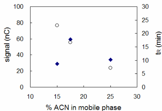
Figure 2-2. Optimizing acetonitrile content in the SDS-containing mobile phase.
