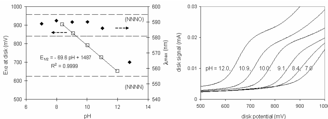
Figure 4-2. pH-dependent spectroscopy and electrochemistry of 1:1 Cu-TRH.
