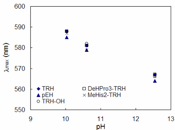
Figure 3-8. Band shift of Cu(II) complexes of TRH analogs with increasing pH.
